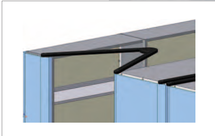
Electrical wires are placed in the cable conduits on the top of a shelf as arms between the segments
